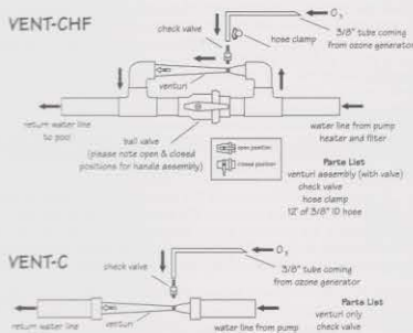
Figure : Water Venturi System
