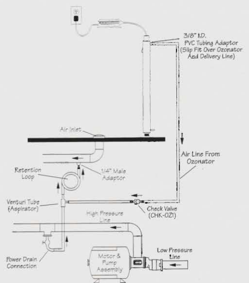
Figure : Pressure Differential System
